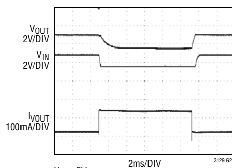
MPPC Response to a Step Load
