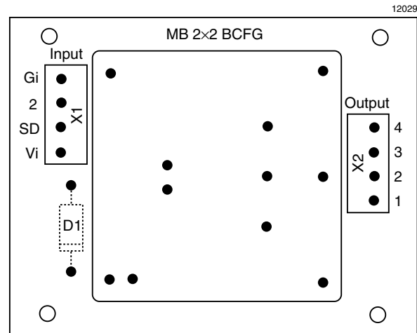
Fig. 7b C/DMB2×2-BCFG print layout
