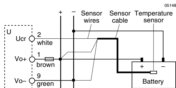
Fig. 3: Connection to the U unit.
