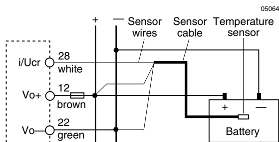
Fig. 2: Connection to the T unit.
