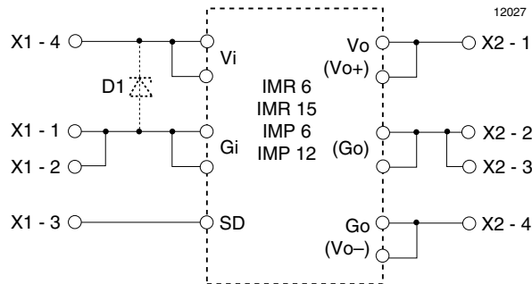
Fig. 7a C/DMB2×2-BCFG circuit diagram
