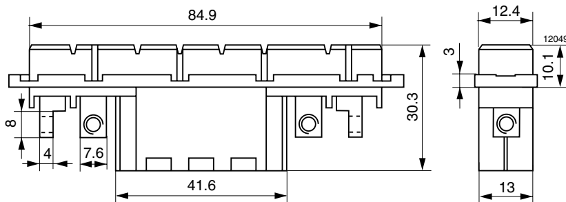
Fig. 13 STV-H15 S4-FSF/CO, Faston cable terminals and four high current screw terminals
