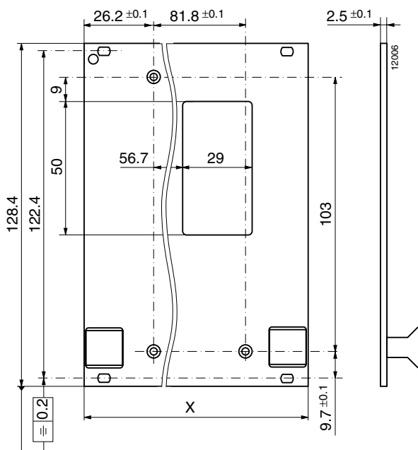
Fig. 5 Front panel for T01 case size
