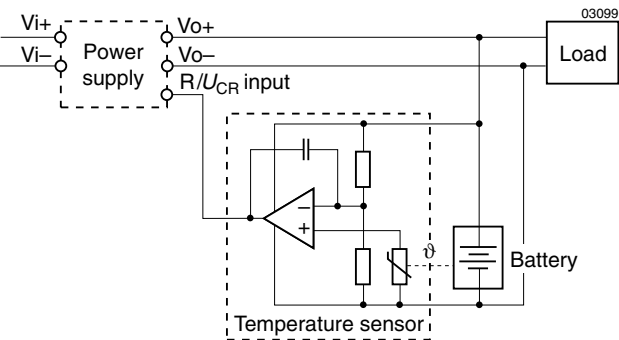
Fig. 1 Functional description
