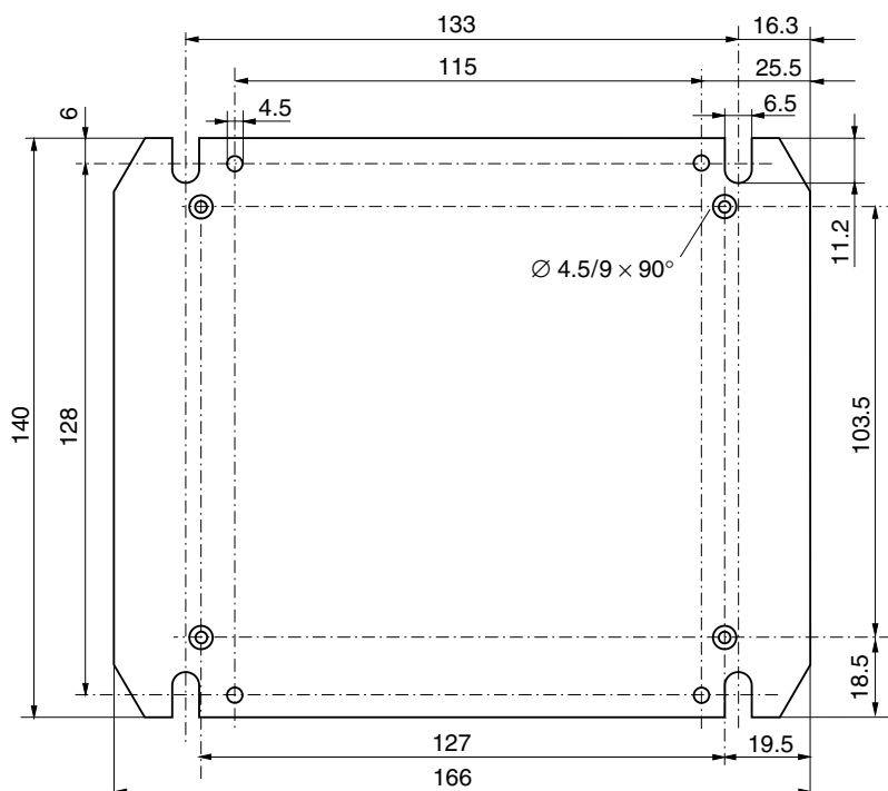
Fig. 1 Mounting plate M Aluminium, black finish
