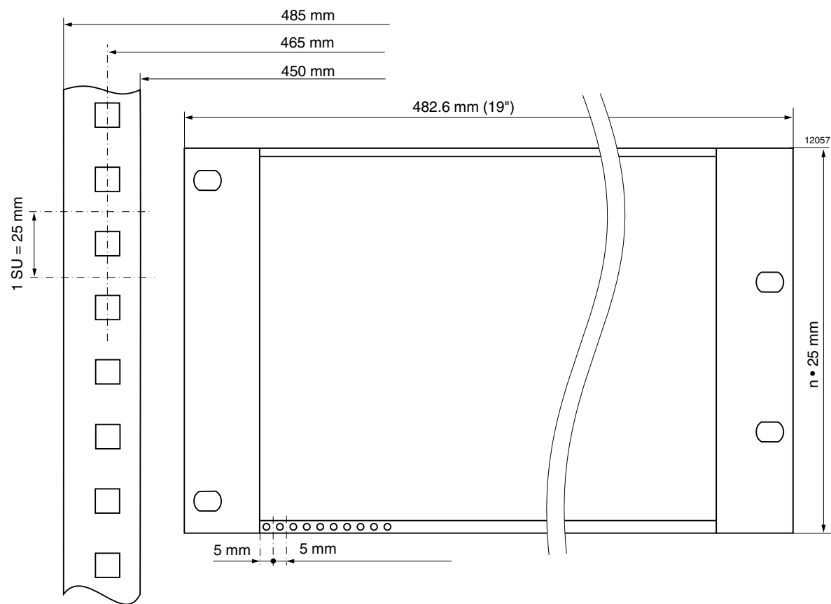
Fig. 2 Metric rack systems
