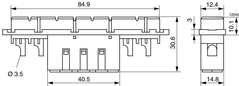
Fig. 12 STV-H15 S4-FLS/CO, screw terminals and four high current soldering terminals
