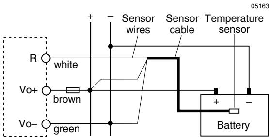
Fig. 5 Connection to a M, H, S, K, KP, LW or OK unit.
