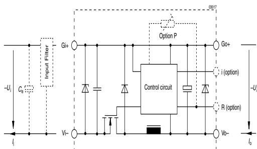
Fig. 3 Single phase configuration L, N 230 V mains: LT-types
