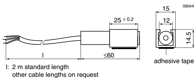
Fig. 4 T and U temperature sensor with mounting fixture.
