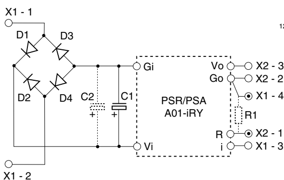
Fig. 6a C/DMBA01- .. circuit diagram
