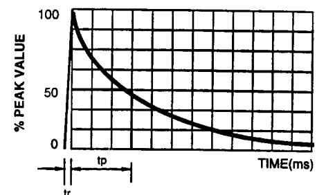
Fig. 3. CURRENT PULSE WAVEFORM
