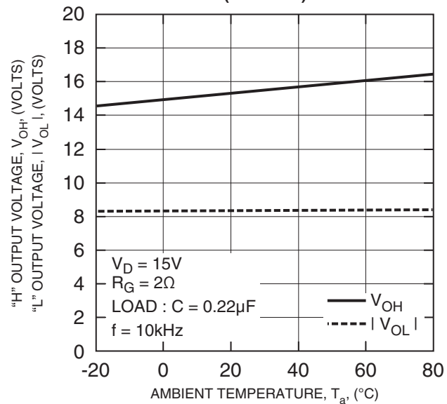
V_{OH} , V_{OL} - T_a CHARACTERISTICS (TYPICAL)
