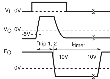
OPERATION OF SHORT CIRCUIT PROTECTION
