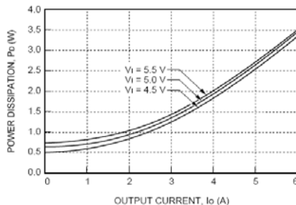
Figure 29. NH020M Power Dissipation vs. Output current.
