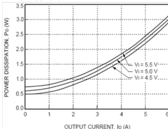
Figure 30. NH020Y Power Dissipation vs. Output Current.
