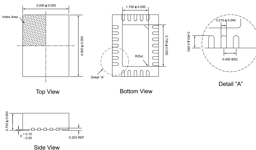
TQFN34-24 3
