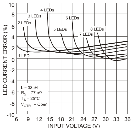
Figure 29. LED Current Deviation vs. Input Voltage
