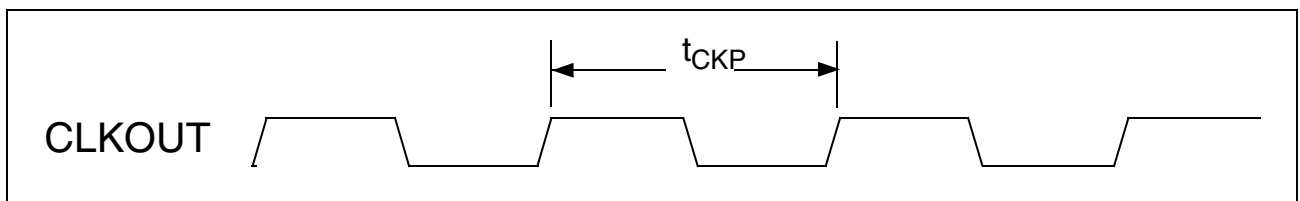
Figure 88 CLOCKOUT Timing
