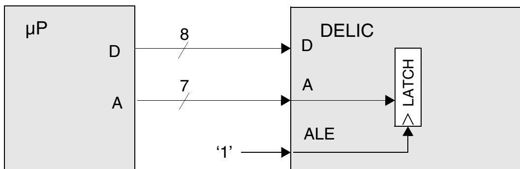
Figure 20 DELIC in Multiplexed and in De-Multiplexed Bus Mode
