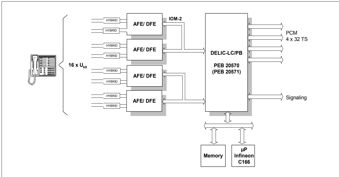
Figure 5 DELIC-LC/PB in Uk0 Line Card for 16 Subscribers
