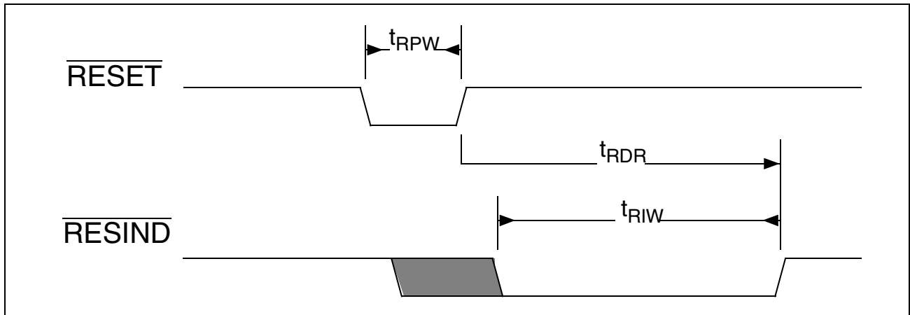
Figure 87 Reset Indication Timing
