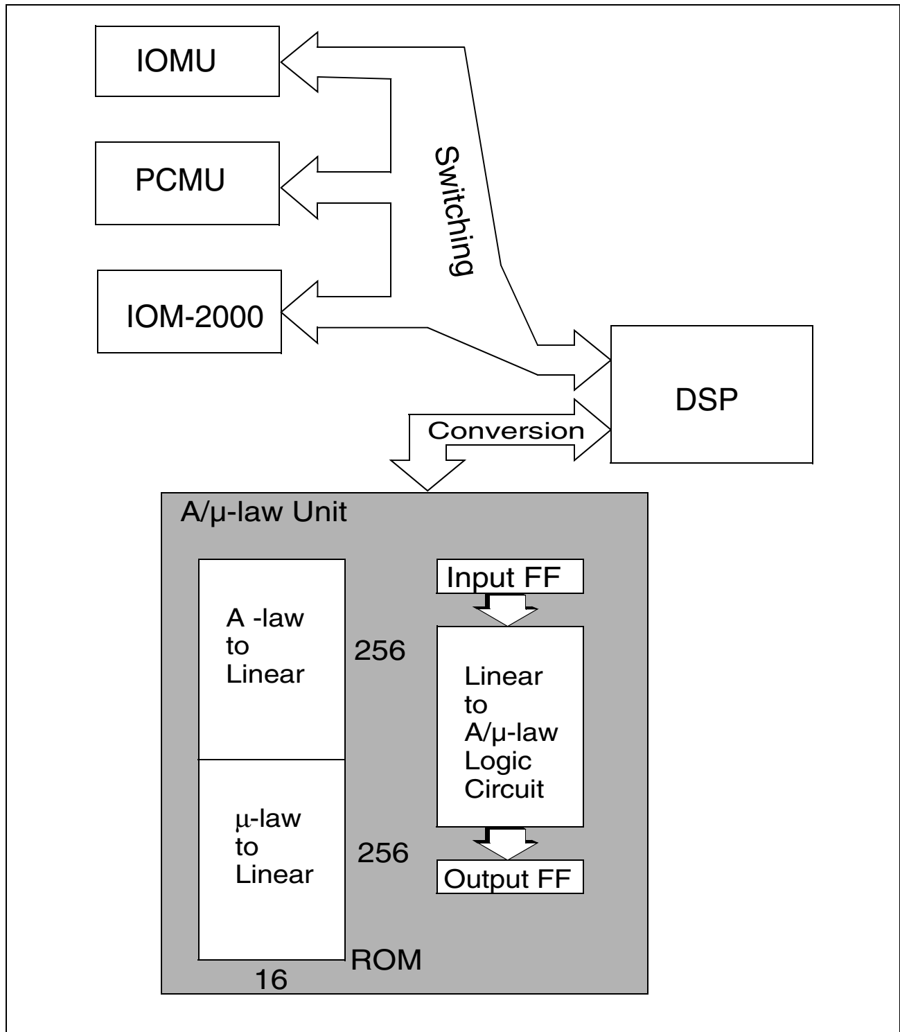
Figure 43 A-/μ-law Unit Integration
