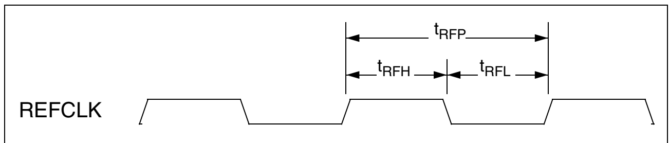
Figure 91 REFCLK Timing
