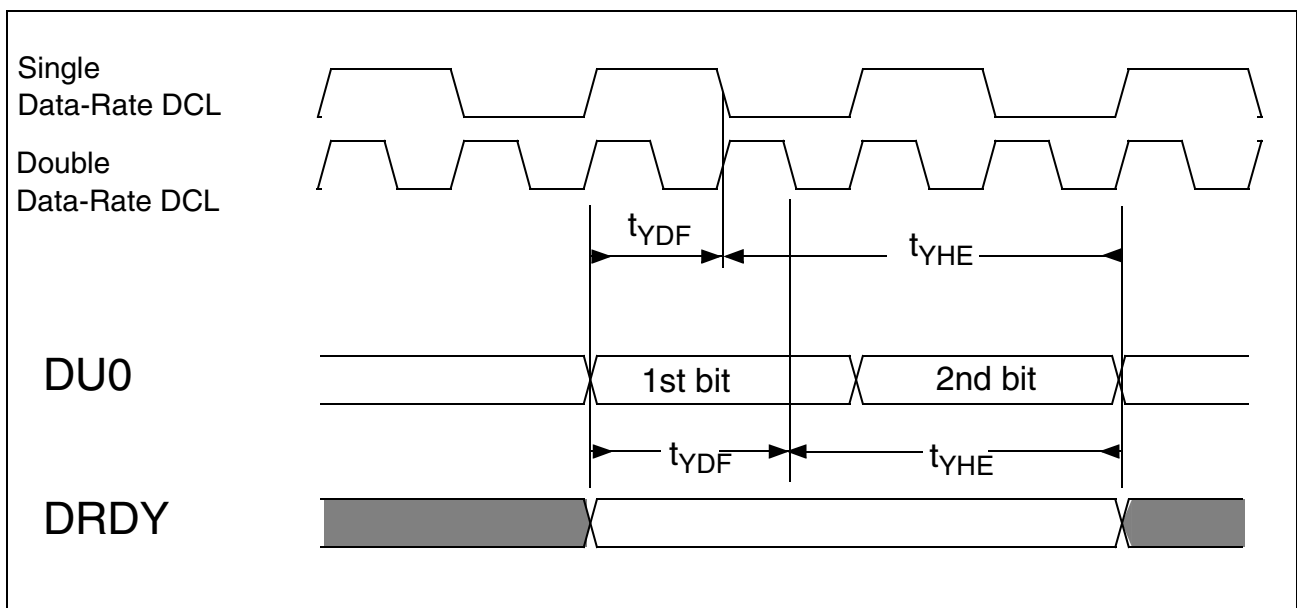
Figure 73 DRDY Timing
