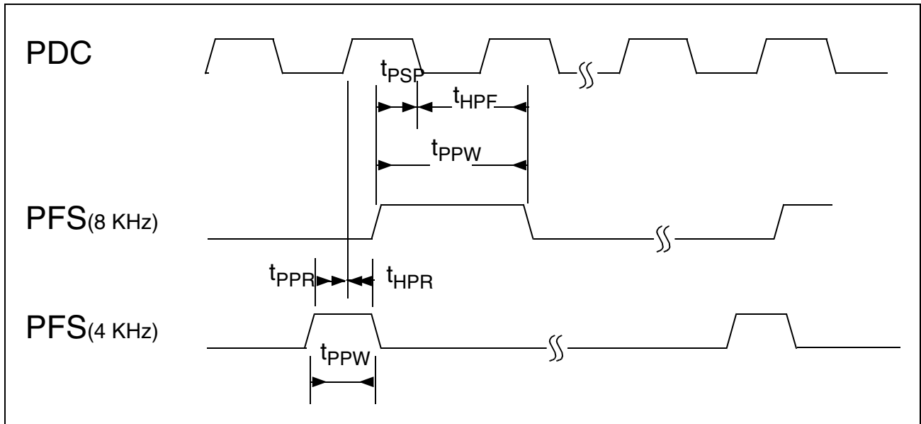
Figure 76 PFS Timing in Slave Mode (Input PCM Clocks)
