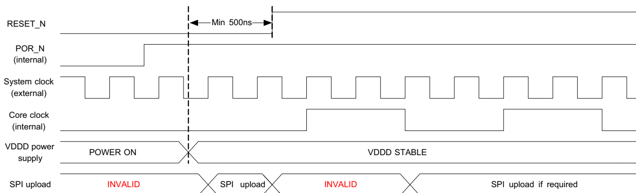
Figure 23. Startup Timing
