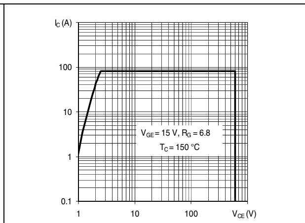
Figure 13. Turn-off SOA
