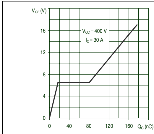
Figure 8. Gate charge vs. gate-emitter voltage
