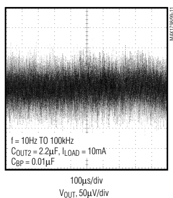
OUTPUT NOISE
