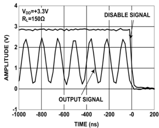
FIGURE 16. DISABLE TIME
