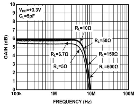
FIGURE 4. GAIN vs FREQUENCY FOR VARIOUS R_{LOAD}
