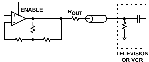
FIGURE 26. DC COUPLE
