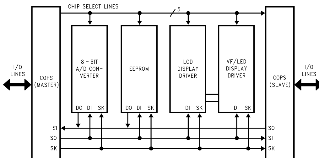
FIGURE 24. MICROWIRE/PLUS Application
