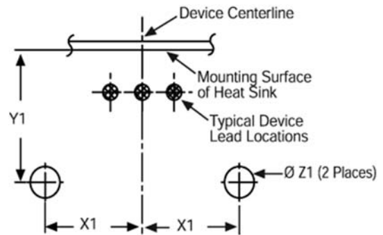
Mounting Details:
