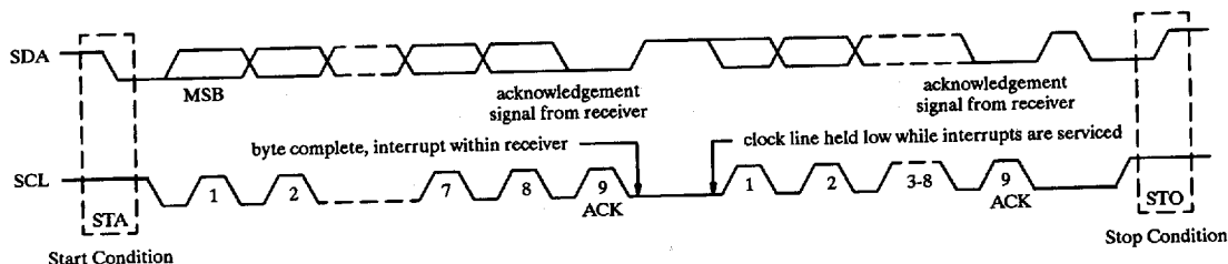
Figure 9. Data Transfer on the I 2 C Bus
