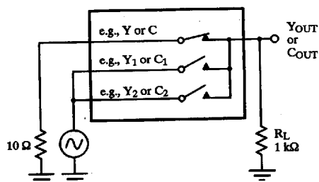
Figure 2. Component Crosstalk
