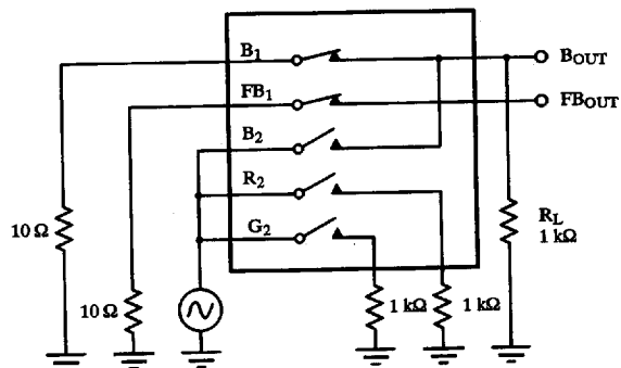
Figure 3. Channel Crosstalk
