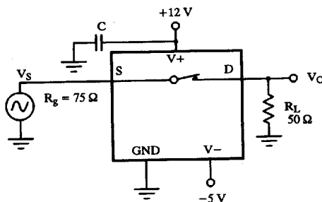
Figure 4. Bandwidth
