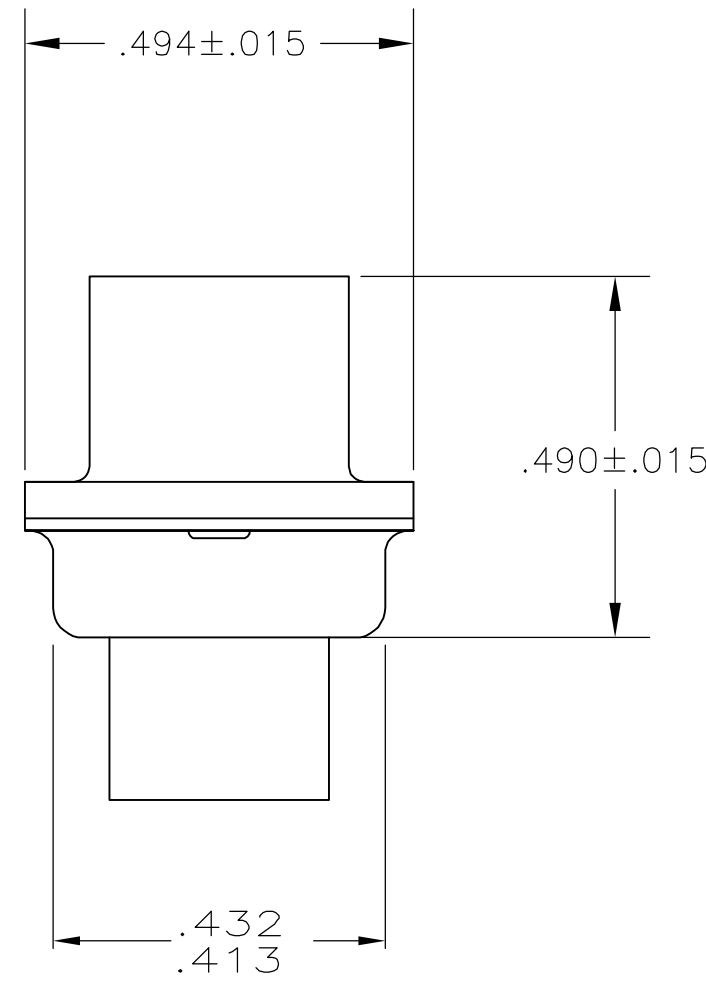
VIEW FOR -1 THRU -4
