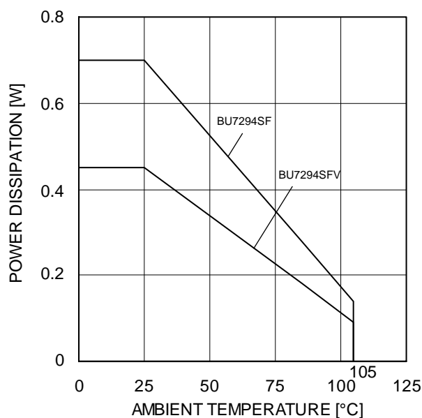
Figure 26. Derating curve
