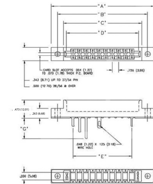
IN-CONTACT POLARIZING KEY
