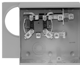
200 Ampere Single-Position Meter Socket (1004884ARHCH)
