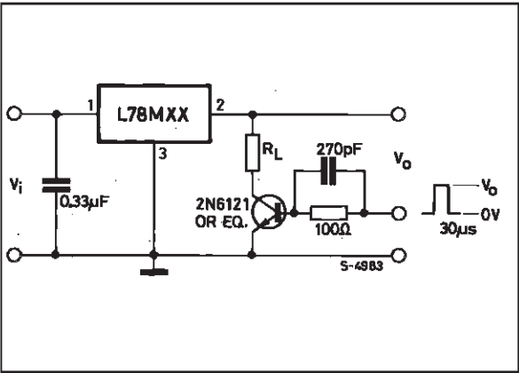
Figure 2 : Load Regulation.
