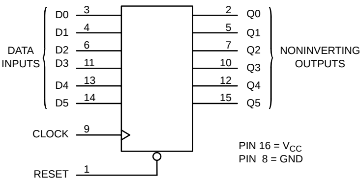
Figure 2. Logic Diagram
