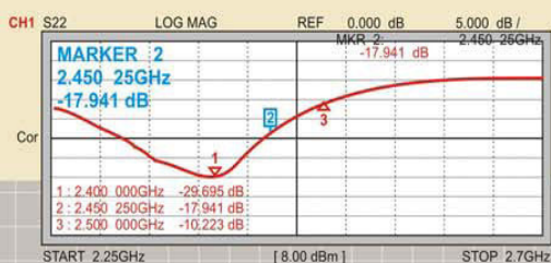
Return Loss
