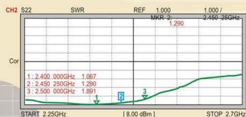
SWR
