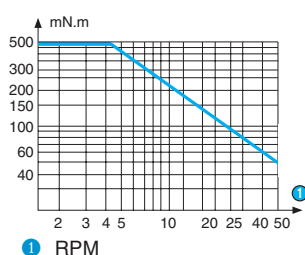
Graph of torque versus speed 82 514 0
