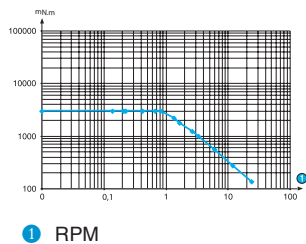
Torque / speed curves 80 513 5
