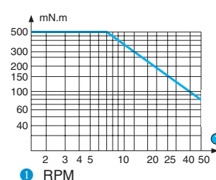
Graph of torque versus speed 82 514 5
