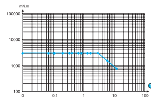
Torque / speed curves 80 533 0
