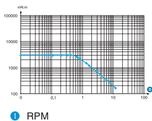
Torque / speed curves 80 513 0
