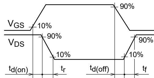
Waveform
