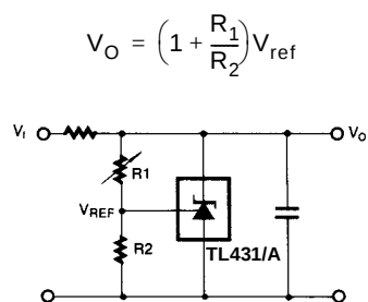
Figure 10. Shunt Regulator
