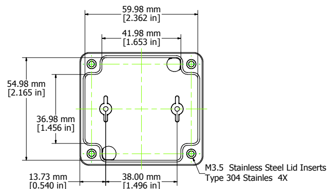
BOX - INSIDE
