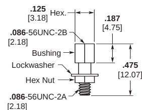
Part Number 5-1532137-9 Jackpost Assembly (P) S96-0002-0009 M83513/5-07
