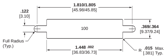
Front Mounting
