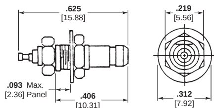
8-32 UNC-2A (Modified) Receptacle, Rear Mount Part Number 145-0003-0001
