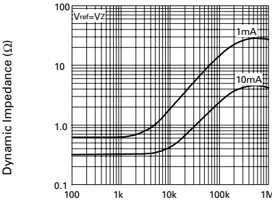
Dynamic Impedance v Frequency
