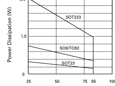
Power Dissipation Derating
