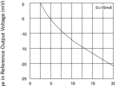
Change in Vref v Cathode Voltage
