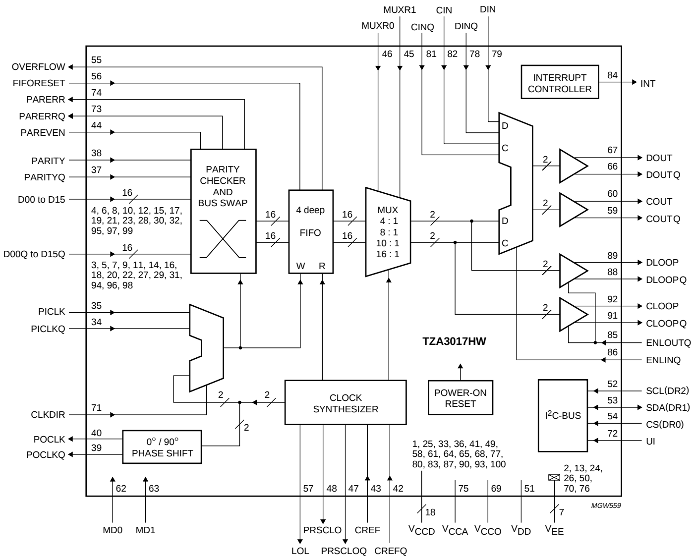
Fig.1 Simplified block diagram.
