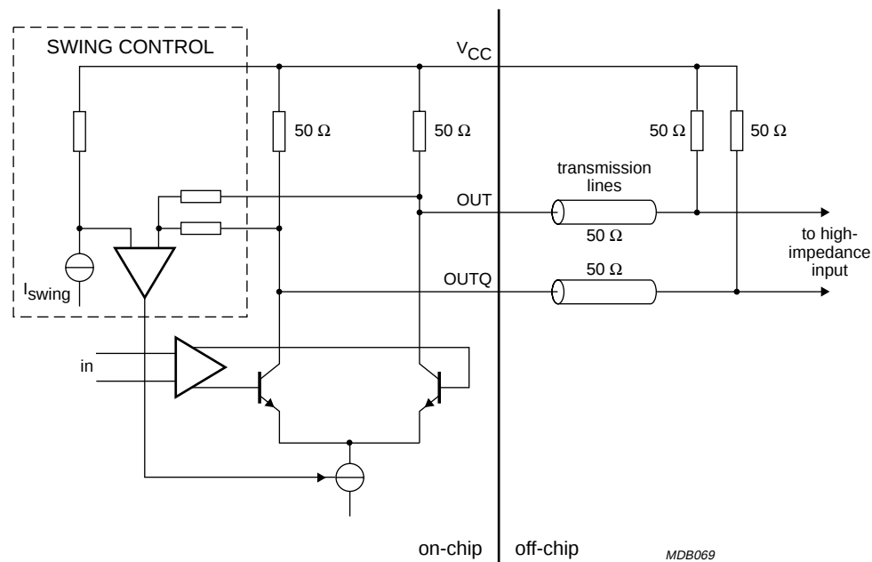
Fig.28 Serial output CML mode (DC-coupled).
