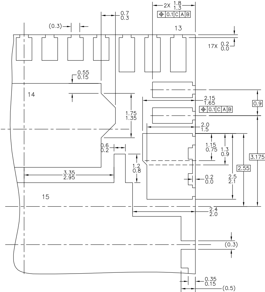
DETAIL H
