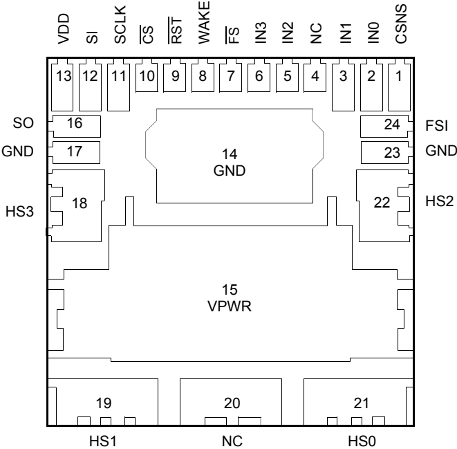
Figure 19. Pin Connections
