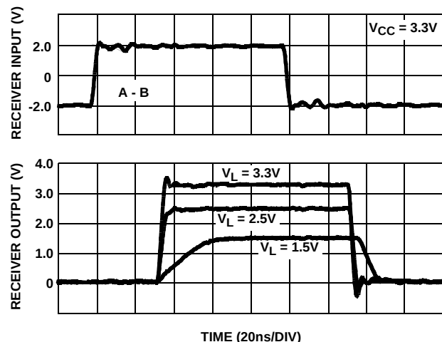
FIGURE 16. RECEIVER WAVEFORMS
