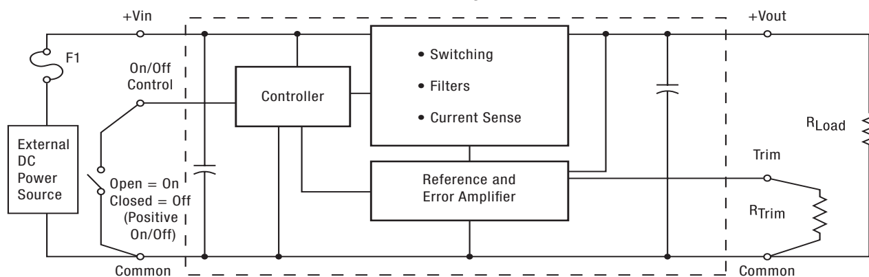
Connection Diagram
