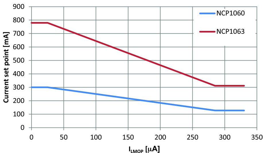
Figure 43. Ipk Set-point Dependence on I_{LMOP} Current
