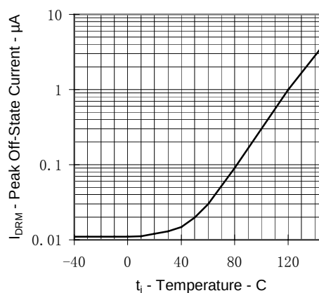
Fig.2 Typical Peak Off-State Current vs Junction Temperature
