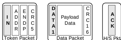
Figure 1-5. An Interrupt Transfer
