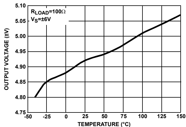
FIGURE 33. OUTPUT VOLTAGE vs TEMPERATURE
