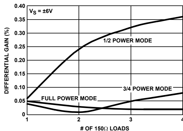
FIGURE 26. DIFFERENTIAL GAIN
