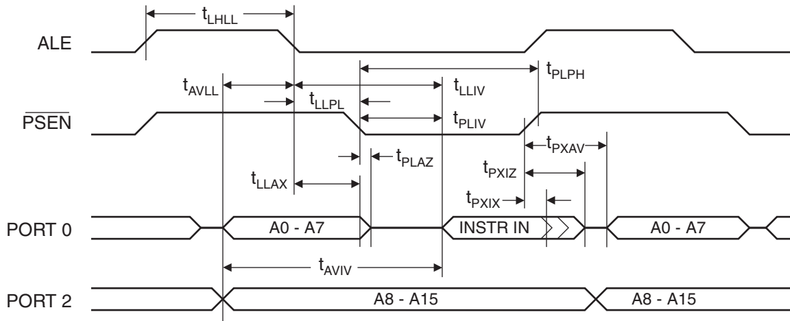
Figure 25-7. External Program Memory Read Cycle
