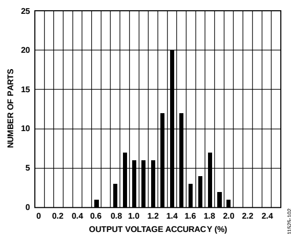
Figure 8. Output Voltage Accuracy at 210^{\circ}\text{C} , FLATPACK Package
