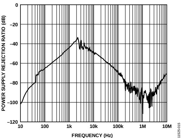
Figure 22. Power Supply Rejection Ratio (PSRR) vs. Frequency, C_{LOAD} = 1 \mu F
