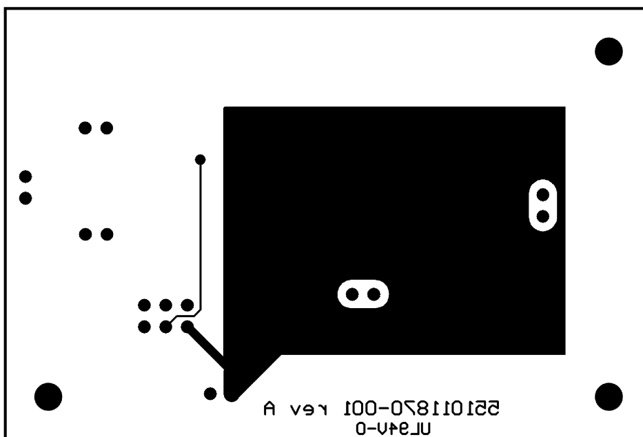
Figure 38. Bottom Layer
