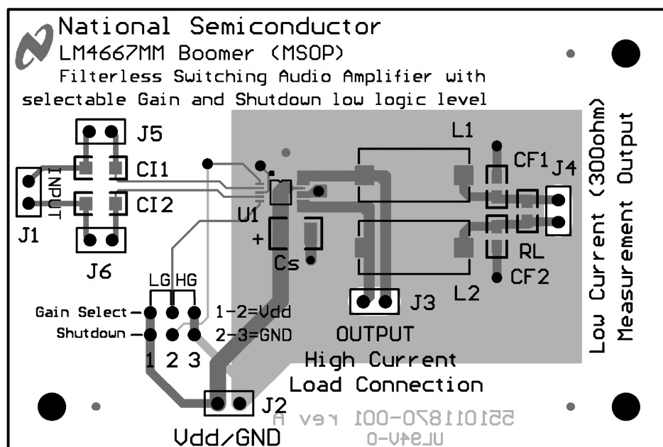
Figure 35. Composite View
