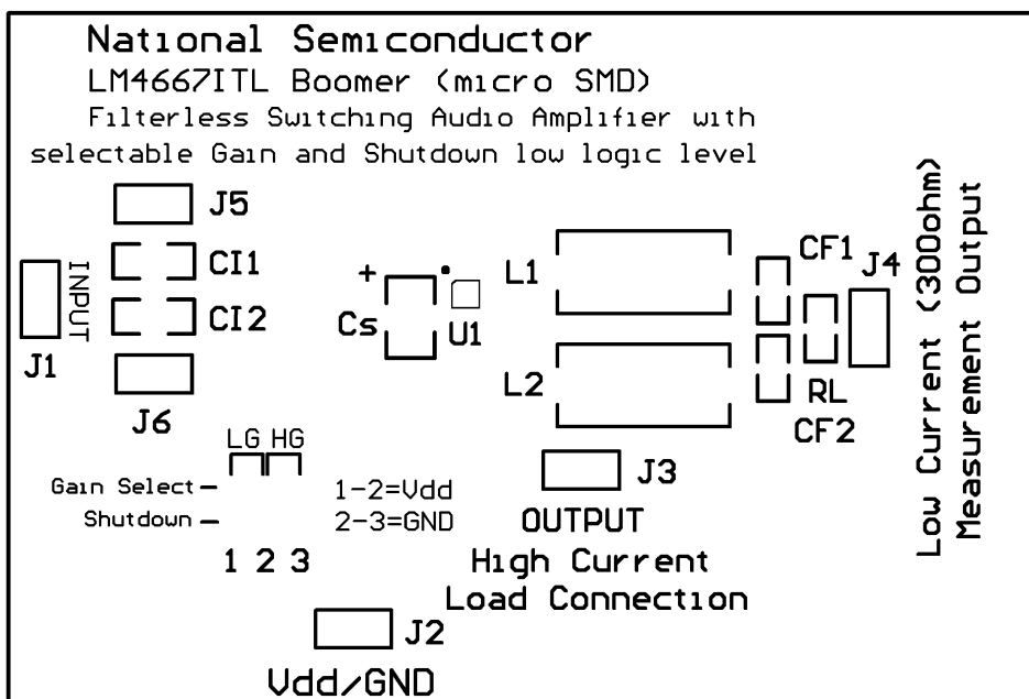
Figure 32. Silk Screen
