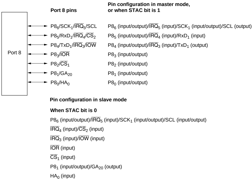
Figure 7.16 Port 8 Pin Configuration
