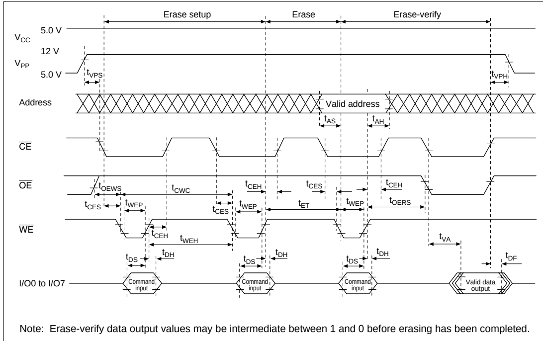
Figure 19.19 Erase Timing
