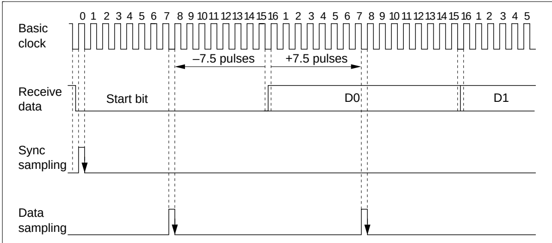
Figure 12.18 Sampling Timing (Asynchronous Mode)
