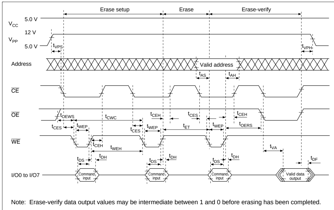
Figure 20.19 Erase Timing
