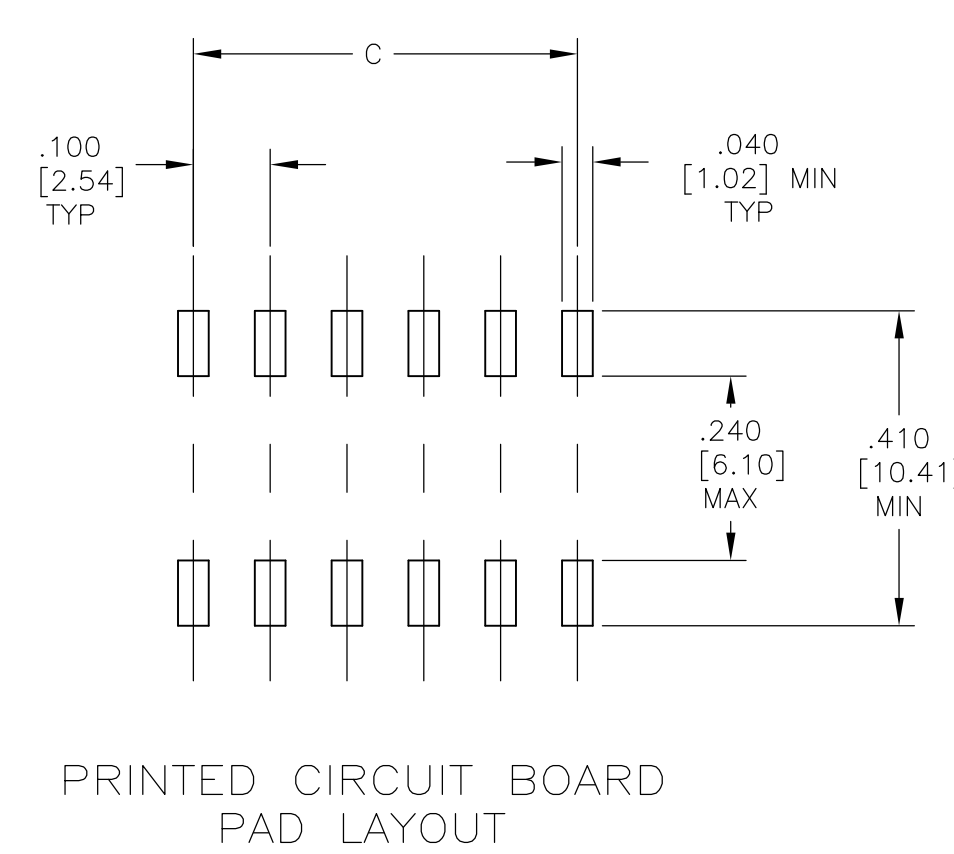
"L" GULL WING TYPE SURFACE MOUNT
