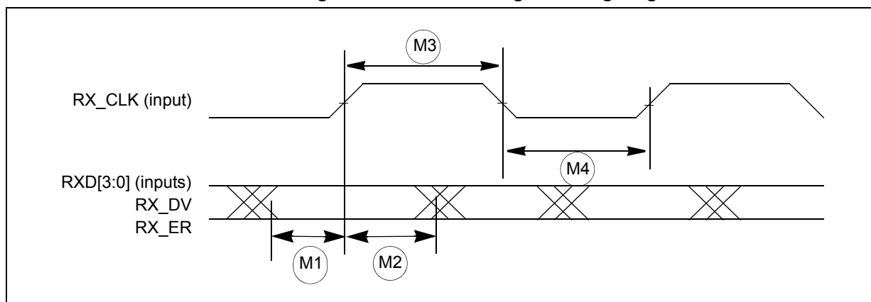
Figure 38. MII receive signal timing diagram
