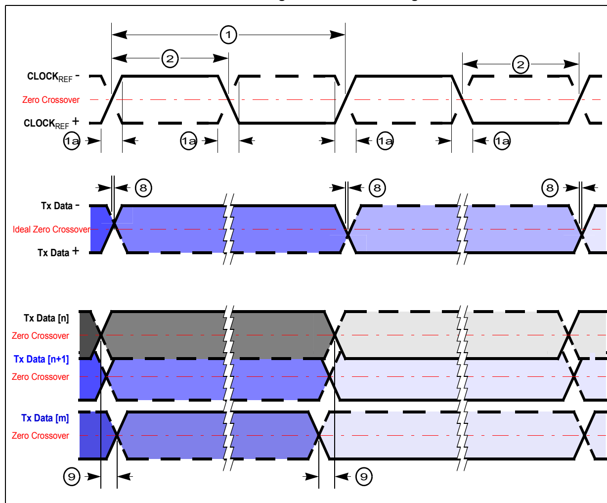
Figure 24. Aurora timings
