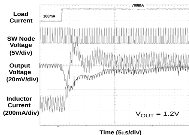
Transient Response
