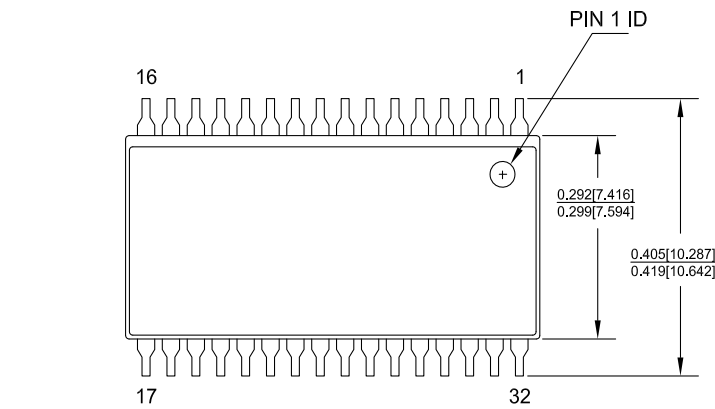
Figure 16. 32-pin SOIC (300 Mil) Package Outline, 51-85127
