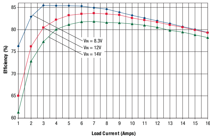
OKY2-T/16-D12 Efficiency vs. Line Voltage and Load Current @ +25°C (V OUT = 1V)
