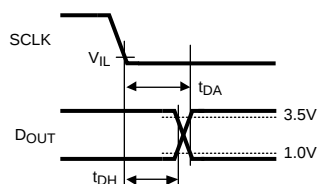
Figure 5. Hold and Access Times
