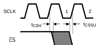
Figure 6. Valid \overline{CS} Assertion Times
