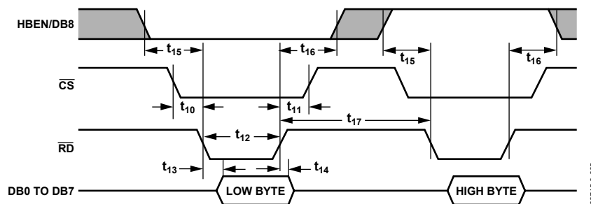
Figure 39. AD7938/AD7939 Parallel Interface—Read Cycle Timing for Byte Mode Operation ( \overline{W/\overline{B}} = 0 )
