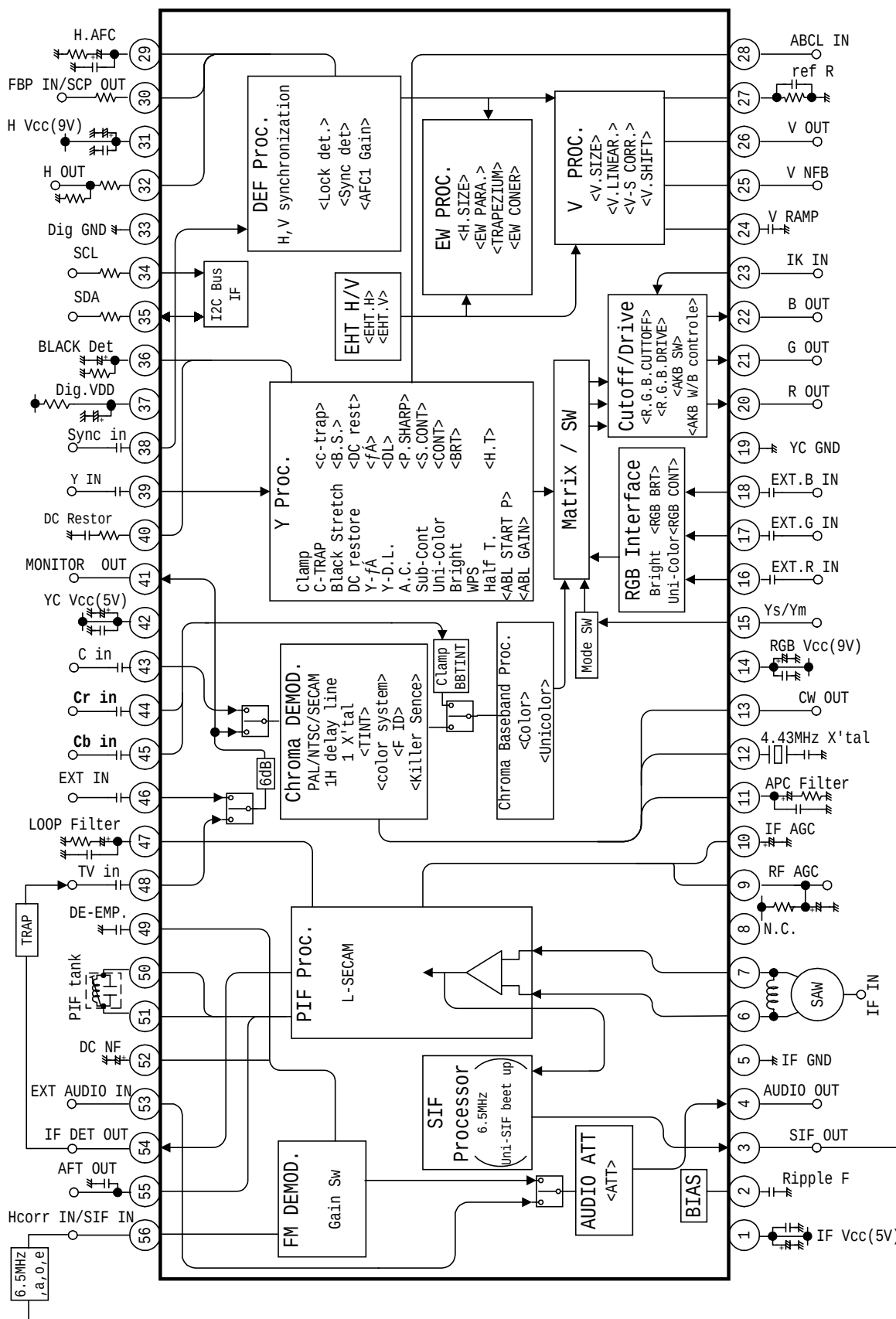
TB1254N BLOCK DIAGRAM
