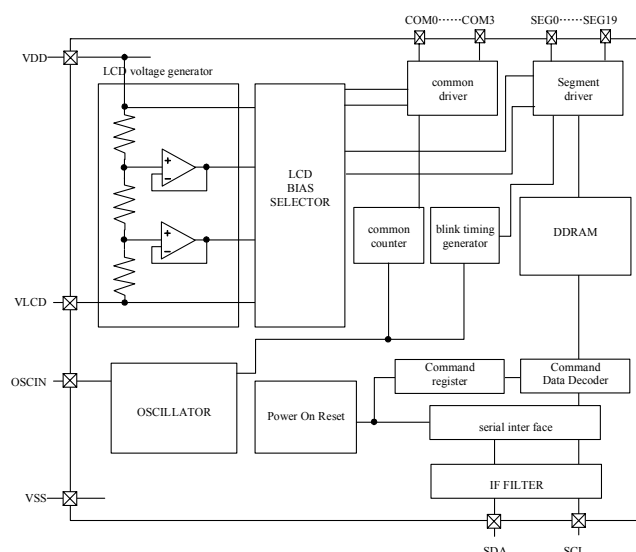
Fig.5 Block Diagram (BU9796FS)
