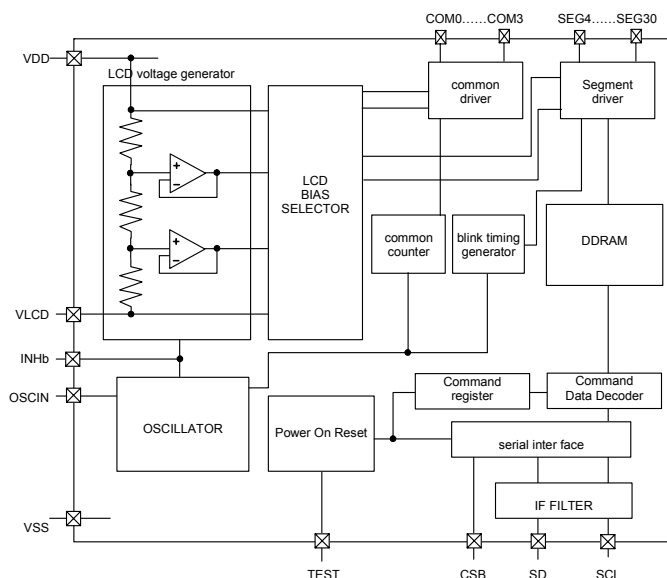
Fig.9 Block Diagram (BU9795AFV)
