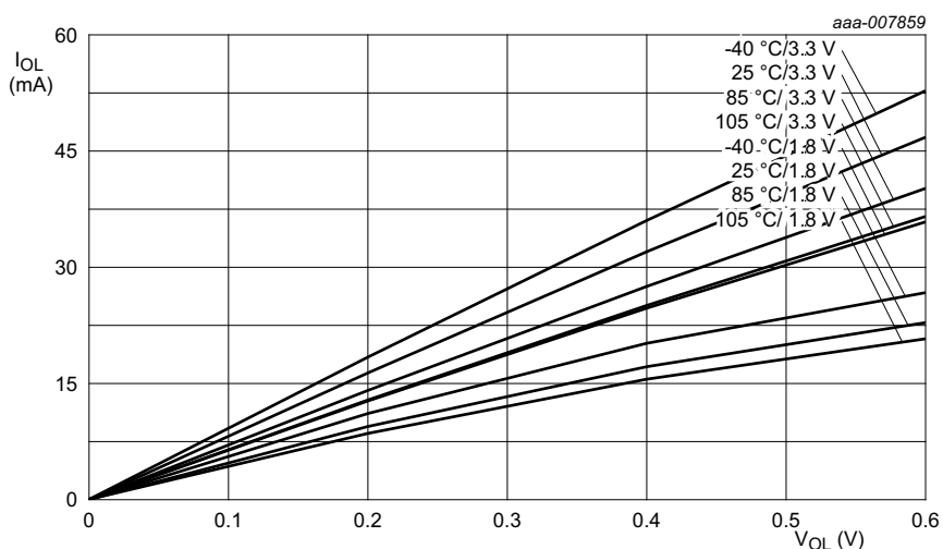
Fig 23. I 2 C-bus pins (high current sink): Typical LOW-level output current I_{OL} versus LOW-level output voltage V_{OL}
