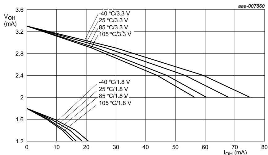
Fig 22. High-drive output: Typical HIGH-level output voltage V_{OH} versus HIGH-level output current I_{OH}
